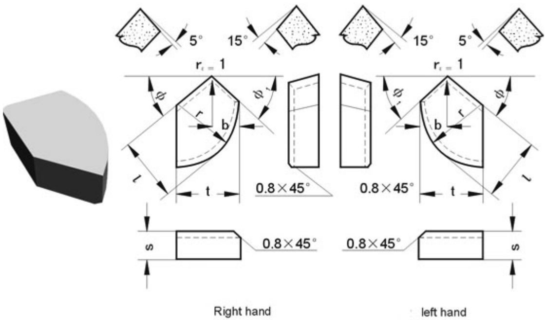
Tungsten carbide brazed tips type A5
